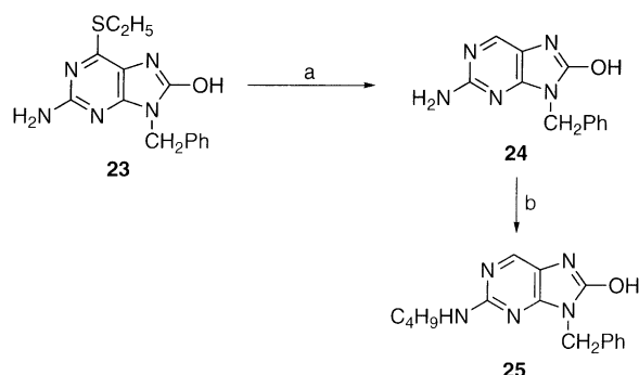
Scheme 5. Reagents and conditions: (a) Raney Ni, NH 4 OH, CH 3 OH, reflux (61%); (b) C 3 H 7 CHO, NaBH 3 CN, CH 3 OH, rt (40%).
