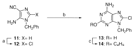
Scheme 2. Reagents and conditions: (a) NCS, THF, rt (87%); (b) H 2 NCONH 2 , neat (78%); (c) C 4 H 9 Br, K 2 CO 3 , DMF, rt (66%).
