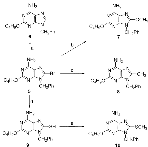
Scheme 1. Reagents and conditions: (a) 10% Pd/C, (C 2 H 5 ) 3 N, H 2 , CH 3 OH, rt (94%); (b) ref 18; (c) Al(CH 3 ) 3 , Ph 3 P, PdCl 2 , THF, reflux (96%); (d) H 2 NCSNH 2 , C 2 H 5 OH, reflux (86%); (e) CH 3 I, K 2 CO 3 , DMF, rt (88%).
