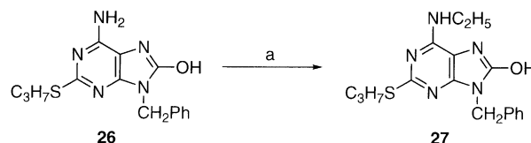
Scheme 6. Reagents and conditions: (a) CH 3 CHO, NaBH 3 CN, CH 3 OH, 50 °C (69%).
