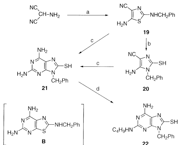
Scheme 4. Reagents and conditions: (a) PhCH 2 NCS, THF, 40 °C, (86%); (b) 5% Na 2 CO 3 , reflux (84%); (c) H 2 NC(NH)NH 2 ·HCl, NaOC 2 H 5 , C 2 H 5 OH, reflux (from 19 : 76%, from 20 : 69%); (d) C 3 H 7 CHO, NaBH 3 CN, CH 3 OH, rt (72%).
