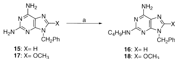
Scheme 3. Reagents and conditions: (a) C 3 H 7 CHO, NaBH 3 CN, CH 3 OH, rt ( 16 : 84%, 18 : 85%).
